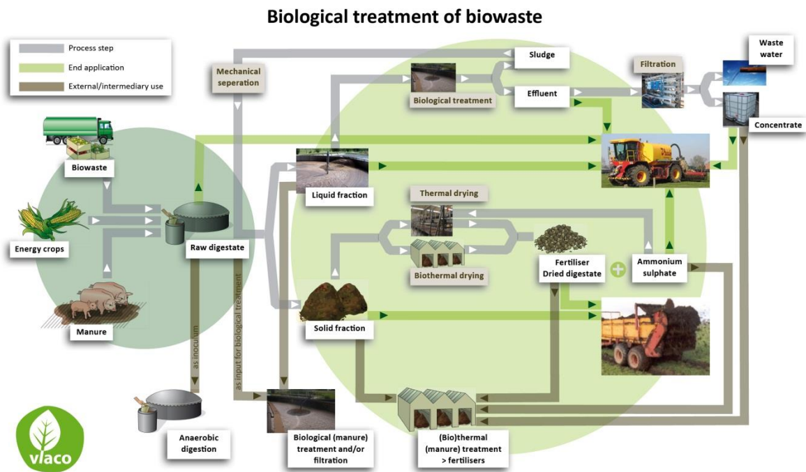
FIGURE 2: Biological treatment of biowaste through anaerobic digestion
