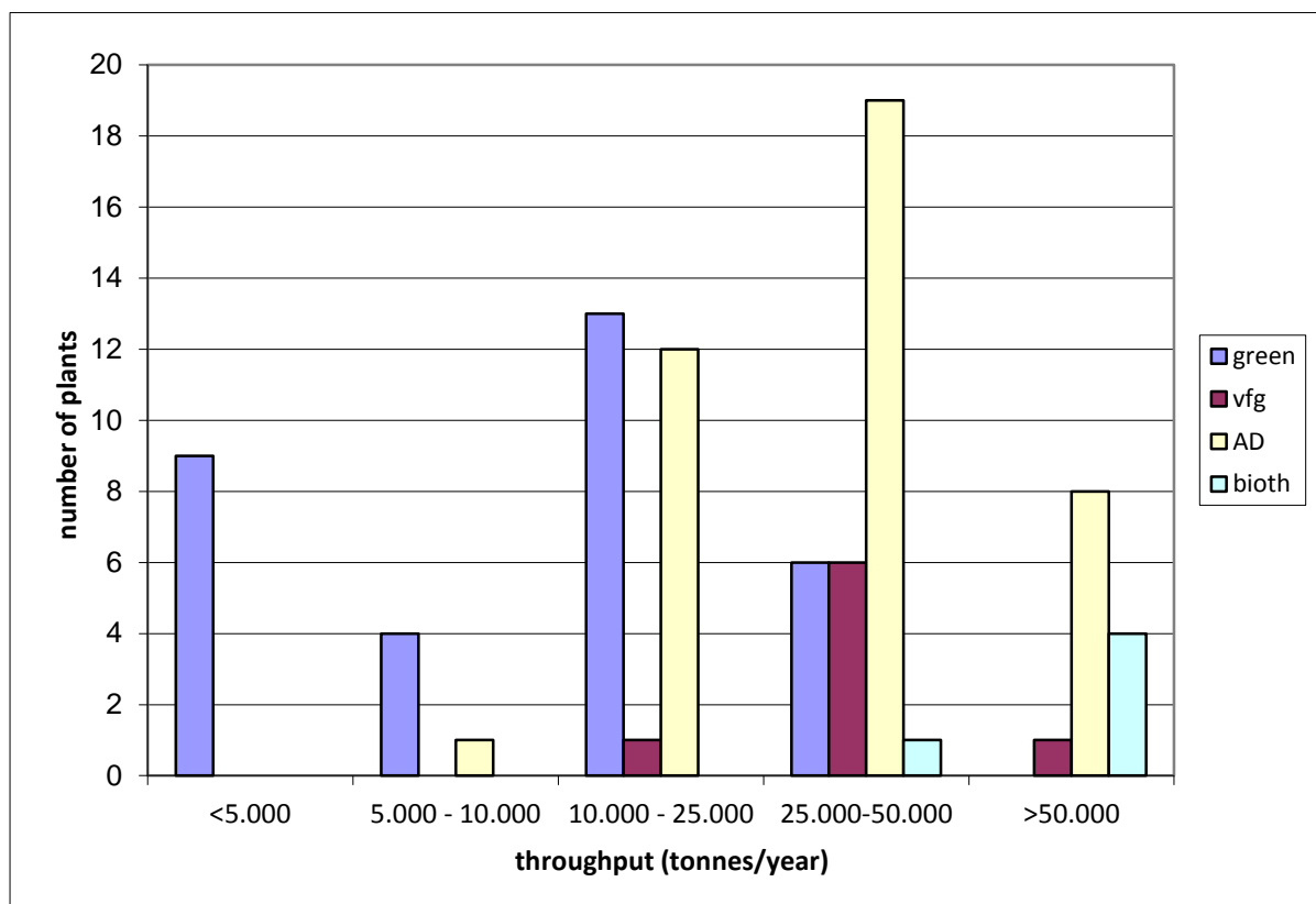
FIGURE 7: Number of plants per class of throughput per year per type of treatment (2013)
